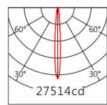
XP-E2 10° 2700K
